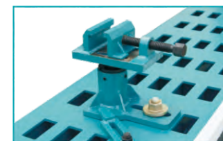
The main clamps design patent
