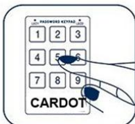
Password keypad
