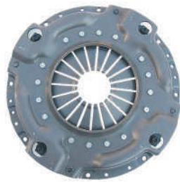
品名: DS400膜片式盖总成 规格: 400*250*379 适配车型: 解放重型车 大柴CA6113BZ 锡柴6110/125ZL3 Product Name:DS400 diaphragm type cover assembly Specification:400*250*379 Fit models:FAW heavy vehicle chaiCA6113BZ xichai 6110/125zl3
