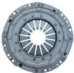
品名: CA330膜片式盖总成 规格: 326*188*365 适配车型: CA142 大柴 锡柴 玉柴 Product Name:CA330 diaphragm type cover assembly Specification:326*188*365 Fit models:CA142 dachai xichai yuchai
