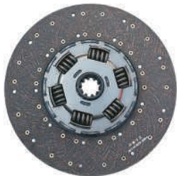
品名: 豪沃430从动盘总成 规格: 430*240*10*52.5 适配车型: 豪沃专用 Product Name: Pull the 430 driven disc assembly Specification: 430*240*10*52.5 Fit models: HOWO
