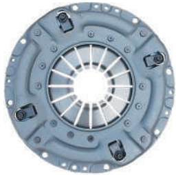
品名: CA151膜片式盖总成 规格: 354*209*381 适配车型: 解放CA151 Product Name:CA151 diaphragm type cover assembly Specification:354*209*381 Fit models:FAW Jie Fang CA151
