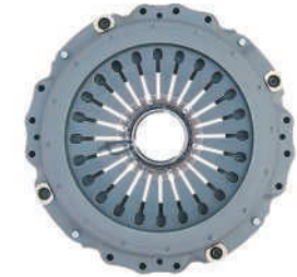
品名: 拉式430 (奔驰) 盖总成 规格: 430*235*450 适配车型: 奔驰CBH Product Name: Pull type 430 (Mercedes Benz) cover assembly Specification:430*235*450 Fit models:Mercedes Benz
