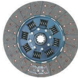
品名: DS400从动盘总成 规格: 400*250*10*44.55 适配车型: 解放重型车 大柴CA6113BZ 锡柴6110/125ZL3 Product Name:DS400 driven disc assembly Specification:400*250*10*44.55 Fit models:FAW heavy vehicle chaiCA6113BZ xichai 6110/125z13
