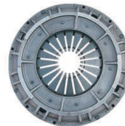
品名: 430铸铁膜片式盖总成 规格: 425*215*450 适配车型: 金龙大客 斯塔尼亚 Product Name: 430 cast iron diaphragm type cover assembly Specification:425*215*450 Fit models:Jinlong Passenger stanyer
