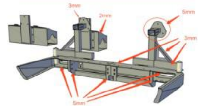
Rear Bumper- D
