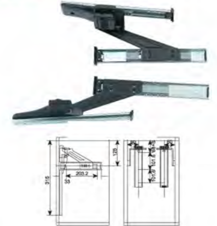
品名: 气压上移门铰 (普通型) Name: Pneumatic up-moving door hinge (Common-type) CG044
