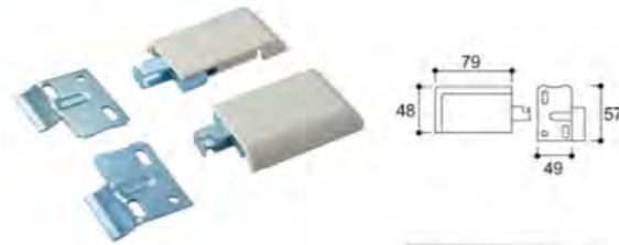
品名：橱柜吊码 Name: Cabinet hanger
