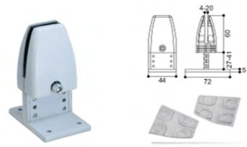
品名：屏风夹 Name: Partition clamp TG113
