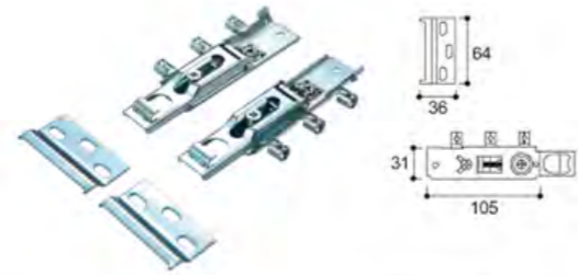
品名：隐藏吊码 Name: Concealed cabinet hanger
