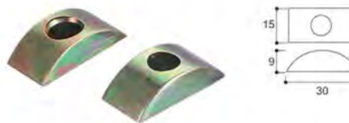
品名：月形垫 Name: Crescent mat LJ082
