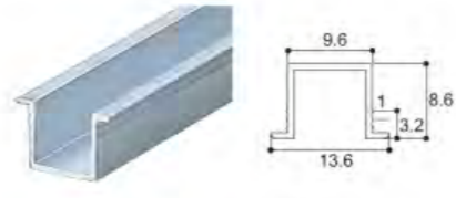
品名：移门轨 Name: Sliding door track
