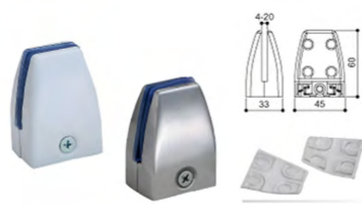
品名：屏风夹 Name: Partition clamp TG115
