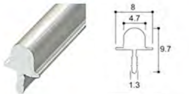
品名：移门轨 Name: Sliding door track
