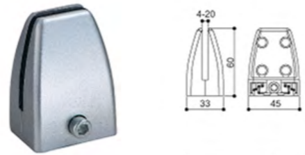
品名：屏风夹 Name: Partition clamp TG117
