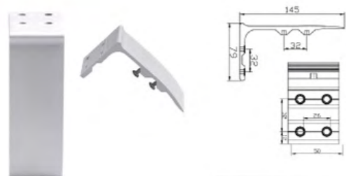
品名：屏风夹 Name: Partition clamp TG118
