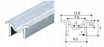
品名：移门轨 Name: Sliding door track
